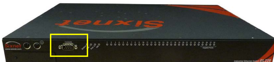
RS232 DB9M Ports (one on each side)
