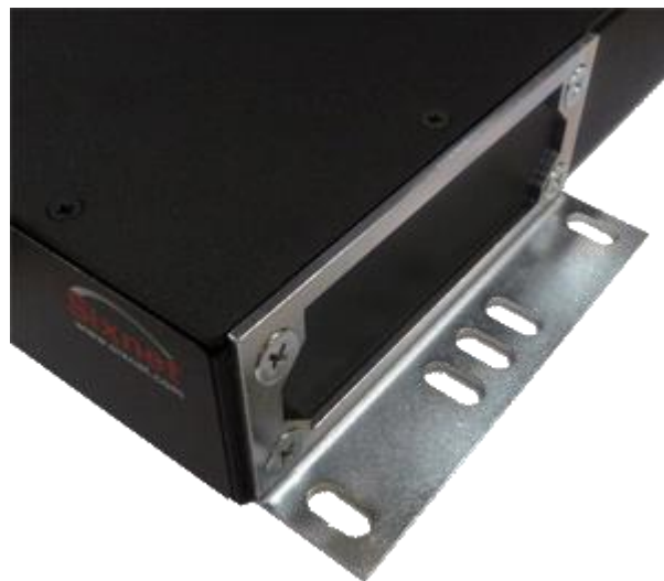
Optional wall bracket Part #: EK1-BRCKT-WALL (set of 2)
