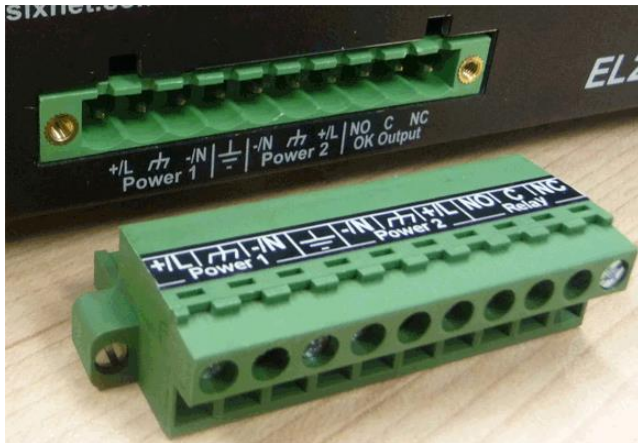
Power Header and Plug Labeling
