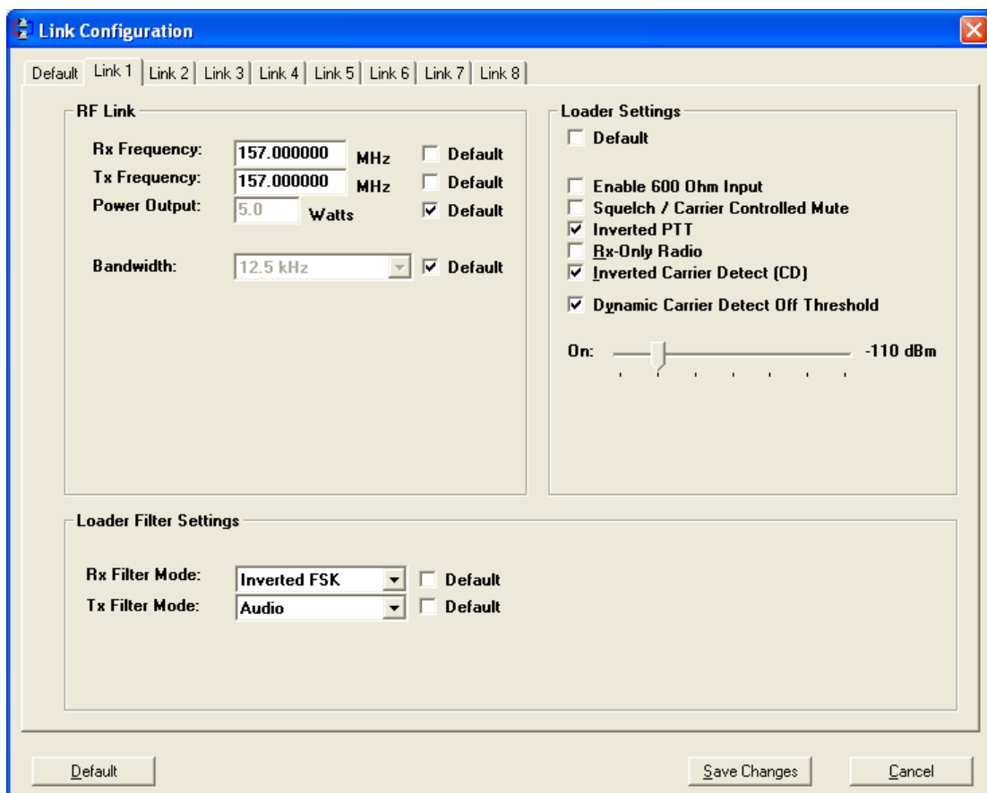
Figure 24 Link Configuration Window – Loader Mode
