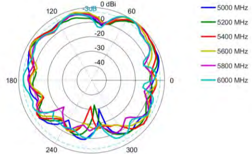
Azimuth: 5000 – 6000 MHz
