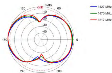
Elevation: 1427 – 1517 MHz
