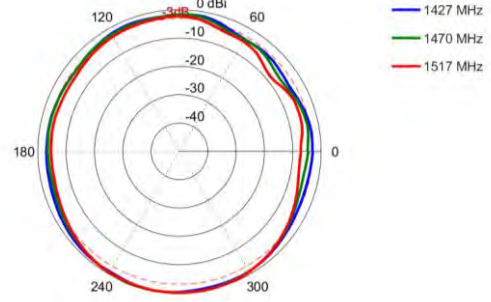
Azimuth: 1427 – 1517 MHz
