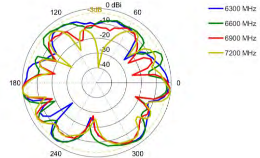
Elevation: 6300 – 7200 MHz
