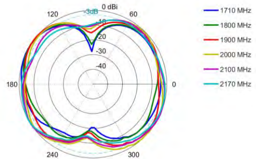
Elevation: 1710 – 2170 MHz
