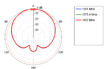
XY Plane: 1561–1602 MHz XZ Plane: 1561–1602 MHz YZ Plane: 1561–1602 MHz
