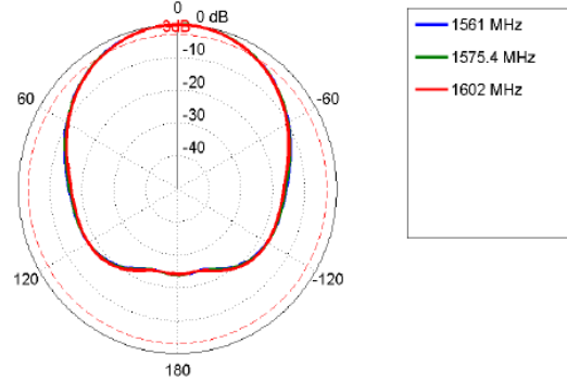
XZ Plane: 1561–1602 MHz
