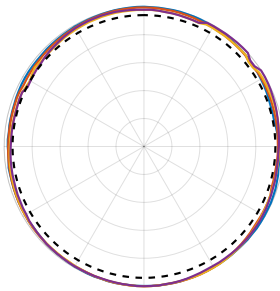
Azimuth (Top View): 2300–2700 MHz
