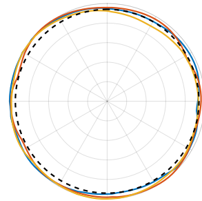
Elevation1 (Side View): 410–470 MHz
