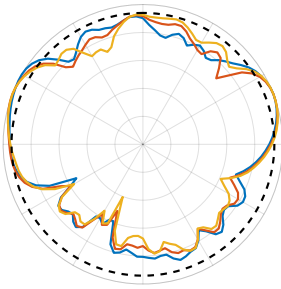
Elevation2 (Side View): 2400–2500 MHz Elevation2 (Side View): 5000–5400 MHz Elevation2 (Side View): 5600–5800 MHz
