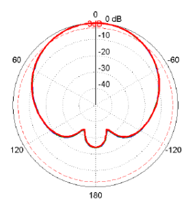
XY Plane: 1561–1602 MHz XZ Plane: 1561–1602 MHz YZ Plane: 1561–1602 MHz
