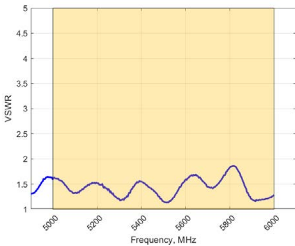
Voltage Standing Wave Ratio (VSWR)
