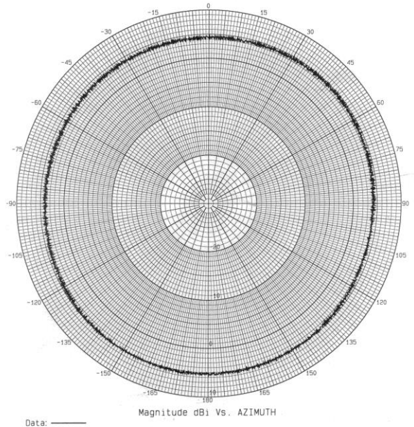
OD5-2400/5500MOD2 – Azimuth Plot @5500 MHz
